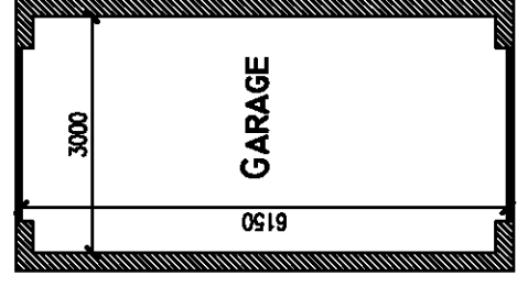
PROPOSED GARAGE FLOOR PLAN @ SCALE 1:100
