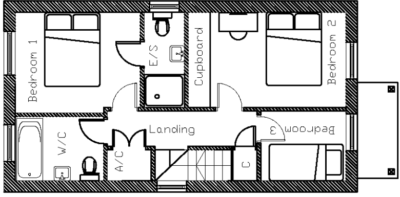
PROPOSED FIRST FLOOR PLAN @ SCALE 1:100
