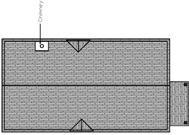
PROPOSED ROOF PLAN @ SCALE 1:100
