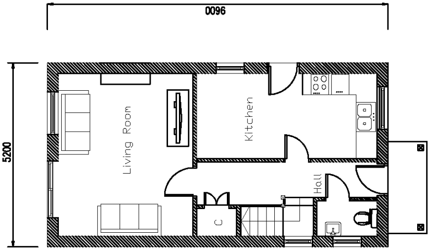
PROPOSED GROUND FLOOR PLAN @ SCALE 1:100
